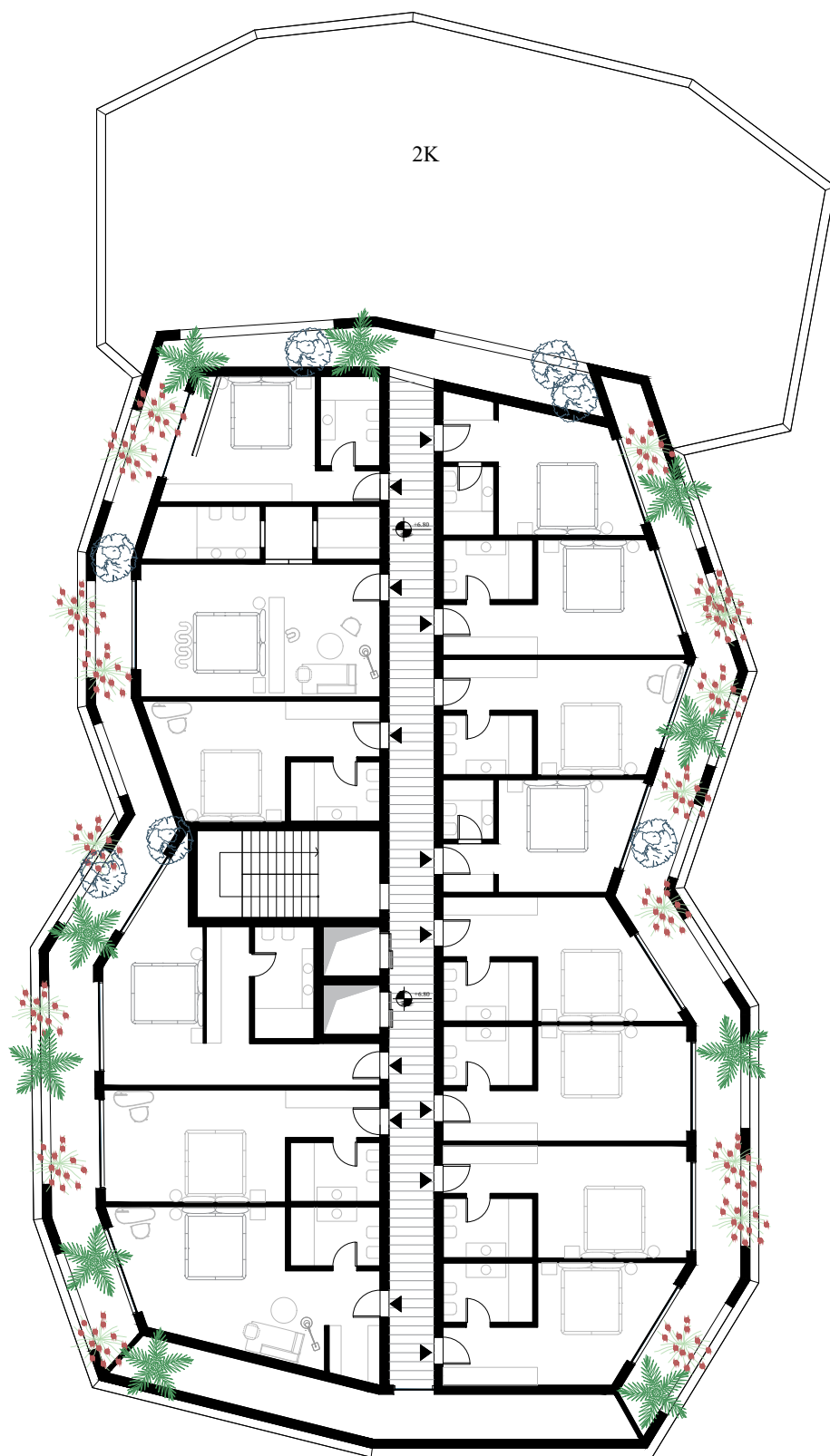
Planimetri Kati 2 / S=776.45m 2
